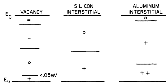
FIG. 23. Schematic diagram of the various charge states of different defects as a function of the position of the Fermi-energy level in the band gap of silicon.
