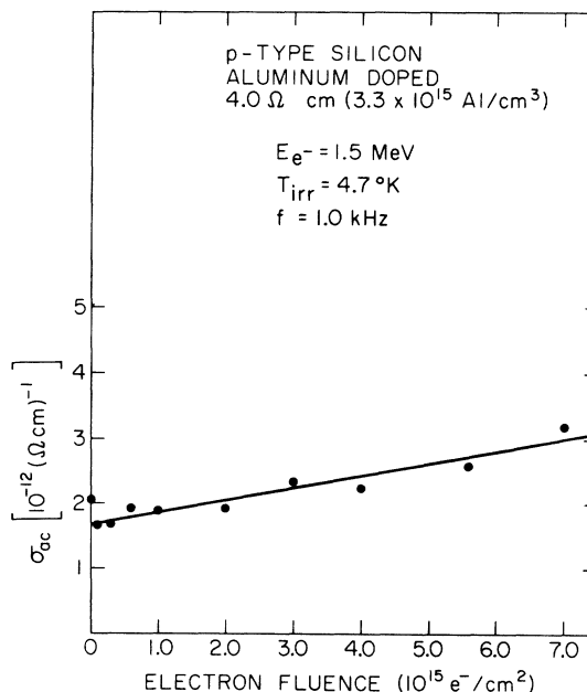
FIG. 3. Changes in \sigma_{ac} with irradiation for 4.0- \Omega -cm p -type silicon, aluminum doped.
