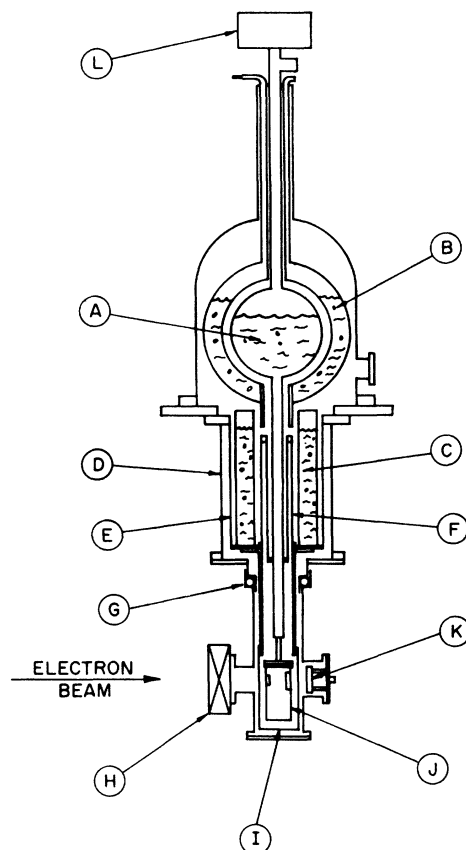
FIG. 1. Schematic of liquid-helium cryostat for electron irradiation studies: (a) 5-liter liquid-helium reservoir; (b) 12-liter capacity liquid-nitrogen reservoir; (c) 7-liter liquid-nitrogen reservoir surrounding tail section of liquid-helium reservoir; (d) rigid tail section; (e) 0.010-in. stainless-steel cylinder supporting liquid-nitrogen reservoir; (f) 0.006-in. stainless-steel concentric cylinders giving liquid-helium tail rigidity; (g) ball-bearing race for rotating Dewar and sample chamber relative to beam; (h) 2-in. gate valve for hook up to Van de Graaff; (i) copper cylinder at liquid-nitrogen temperature with 0.007-in. aluminum-coated Mylar windows for electron beam; (j) sample chamber holding exchange gas around samples and having entrance and exit windows for the electron beam of 0.002-in. Duraluminum; (k) beam stop and beam current monitor mounted on room-temperature cylinder; (l) vacuum-tight enclosure for introduction of exchange gas to the sample chamber and for wire leads running down to the sample.
