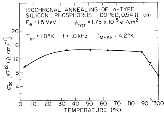
FIG. 17. Isochronal annealing of 0.54- \Omega -cm n -type silicon after irradiation at 1.8°K. Measurements made at reference temperature of 4.2°K.
