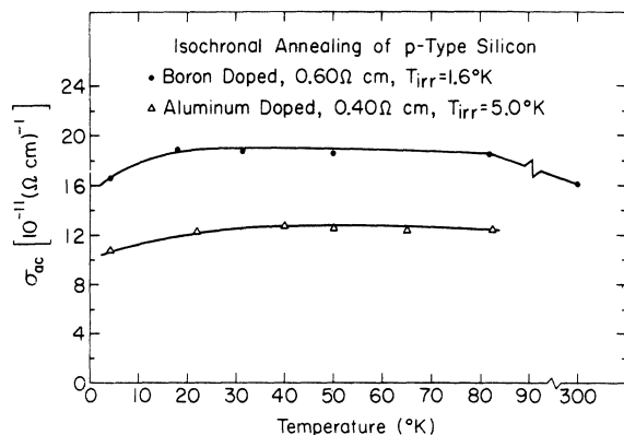
FIG. 12. Isochronal annealing of p -type silicon after irradiation. Measurements made at reference temperature of 4.2°K and frequency of 1 kHz.
