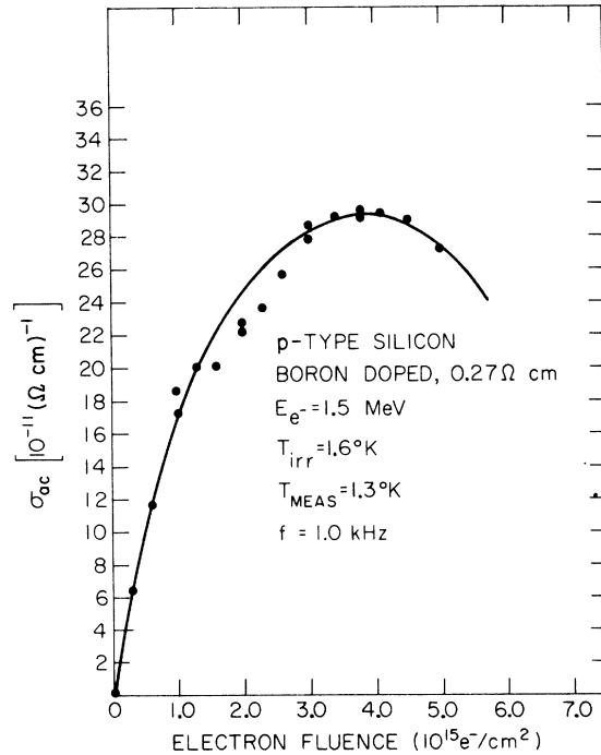
FIG. 10. Changes in \sigma_{ac} produced by irradiation at 1.6°K of 0.27- \Omega -cm boron-doped p -type silicon.
