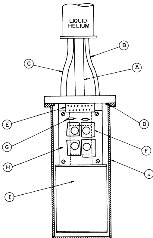
FIG. 2. View of sample mounting chamber: (a) \frac{5}{16} -in.-diam \times 0.006-in.-thick inconel tube carrying exchange gas and lead wires to sample chamber; (b) \frac{1}{8} in.-diam \times 0.004-in.-thick inconel tube carrying liquid helium to the reservoir in sample chamber, with a needle-valve flow control positioned above this tube; (c) \frac{3}{16} -in.-diam. \times 0.006-in.-thick inconel tube for venting helium gas; (d) demountable indium o-ring seal for removing outer cylinder to mount samples; (e) strip of Teflon with copper pins to which wires are attached leading up to top of Dewar and to which wire leads on samples can be readily attached; (f) \frac{1}{16} -in. quartz plate with four silicon samples mounted; (g) carbon resistor thermometer; (h) copper posts \frac{3}{8} \times \frac{3}{16} in. to which quartz plate is mounted and which are hollowed out so that the reservoir can be filled with liquid helium and vented (note that these hollow posts are also filled with liquid helium during irradiation); (i) 1\frac{3}{4} -in.-diam hollow copper cylinder holding a reservoir of 68 cm 3 of liquid helium; the heater wire is wrapped around this cylinder; (j) copper cylinder holding helium exchange gas around samples and having entrance and exit windows for the electron beam of 0.002-in. Duraluminum.
