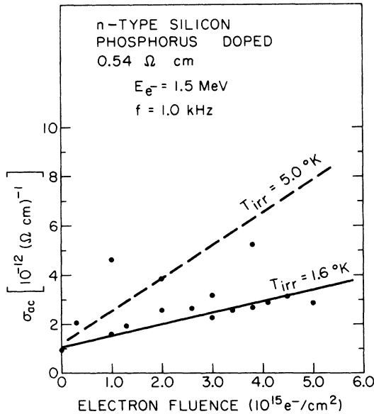
FIG. 15. Comparison of changes in \sigma_{ac} for 0.54- \Omega -cm n -type phosphorus-doped silicon produced at irradiation temperatures of 5.0 and 1.6°K, respectively.
