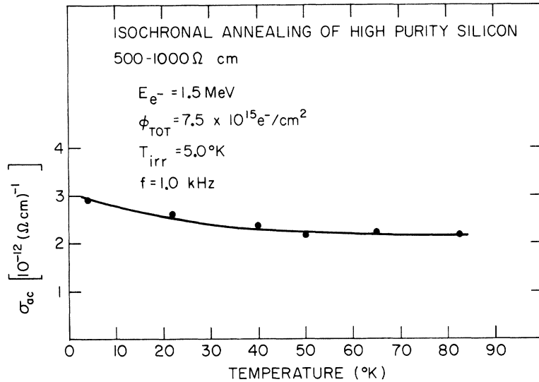
FIG. 22. Isochronal annealing of high-purity silicon after irradiation at 5.0 °K with 1.50-MeV electrons. Measurements made at reference temperature of 4.2 °K.
