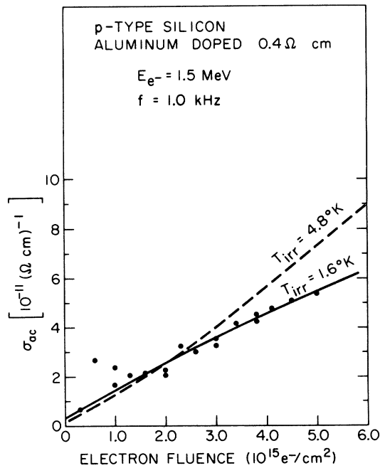
FIG. 8. Comparison of changes in \sigma_{ac} produced at irradiation temperatures of 4.8 and 1.6°K in 0.4- \Omega -cm p -type aluminum-doped silicon.
