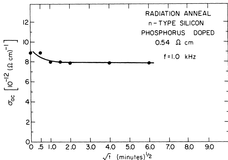
FIG. 19. Damage introduced by 2.00-MeV electron beam at 4.8°K. Looked for radiation annealing effects at 5.0°K using 0.500-MeV electron beam. t is the time in minutes that the 0.500-MeV beam was on.
