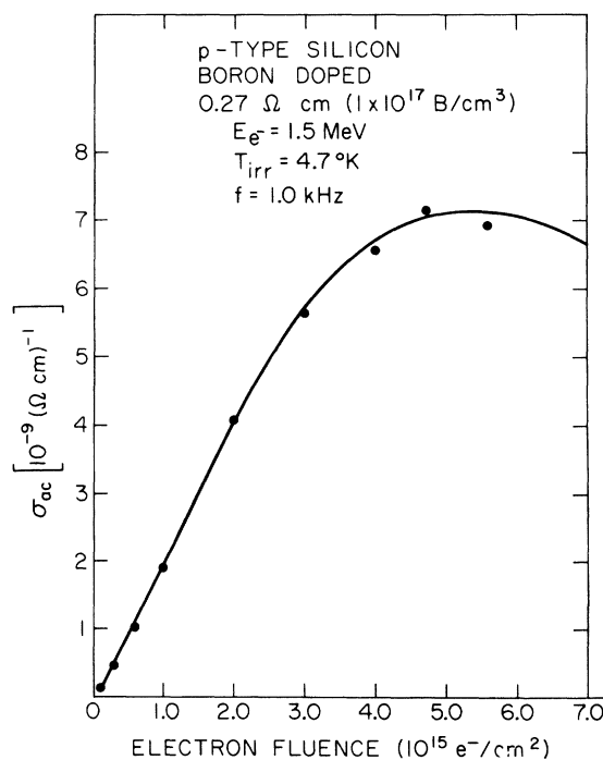
FIG. 5. Changes in \sigma_{ac} with irradiation for 0.27- \Omega -cm p -type silicon, boron doped.
