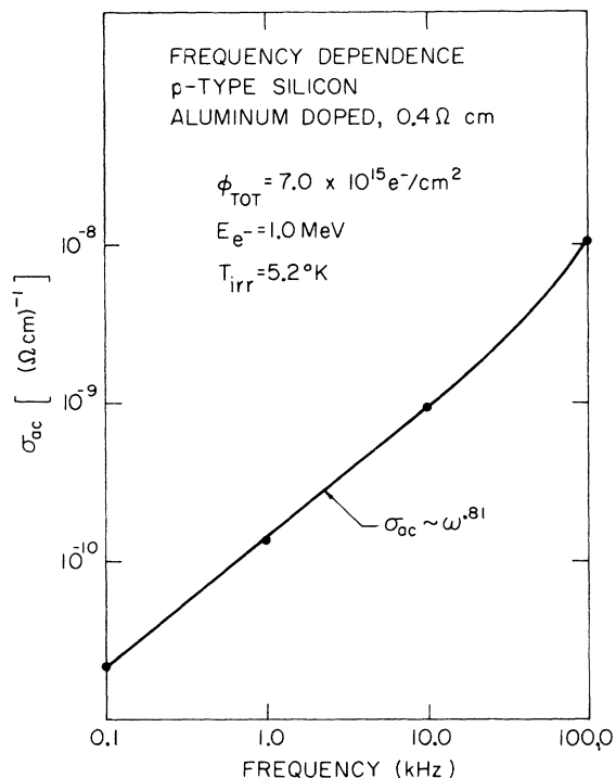
FIG. 6. Frequency dependence of \sigma_{ac} after irradiation of 0.4- \Omega -cm p -type silicon, aluminum doped.
