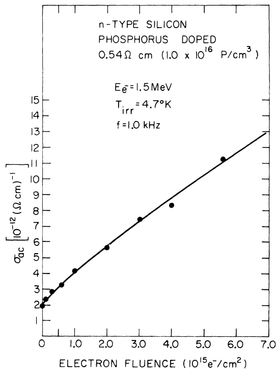
FIG. 14. Changes in \sigma_{ac} in 0.54- \Omega -cm phosphorus-doped n -type silicon caused by irradiation with 1.5-MeV beam.
