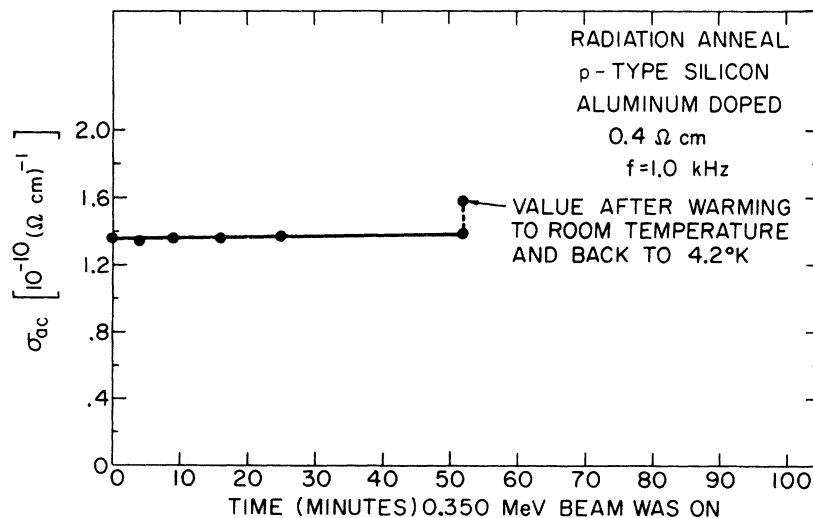
FIG. 7. Damage introduced by 1.0-MeV electron beam at 5.2 °K. Looked for radiation annealing effects at 5.8 °K using 0.350-MeV electron beam at 2.0 \times 10^{-8} A/cm 2 .
