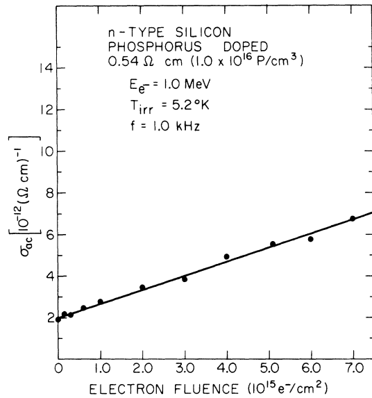
FIG. 13. Changes in \sigma_{ac} with irradiation for 0.54- \Omega -cm n -type silicon doped with phosphorus.
