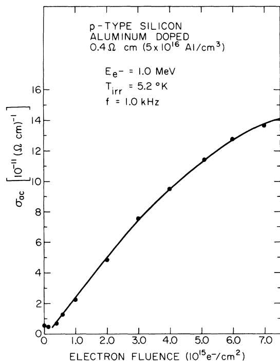
FIG. 4. Changes in \sigma_{ac} with irradiation for 0.4- \Omega -cm p -type silicon, aluminum doped.
