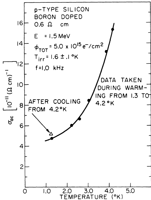
FIG. 11. Magnitude of \sigma_{ac} at various temperatures measured during warming from 1.3°K to 4.2°K and back to 1.3°K at end of irradiation.
