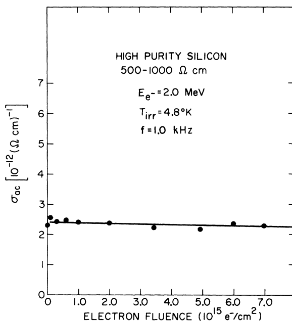
FIG. 21. Measurements of ac hopping conductivity in high-purity silicon irradiated at 4.8°K with 2.0-MeV electrons.
