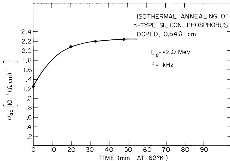
FIG. 18. Isothermal annealing of 0.54- \Omega -cm n -type silicon after irradiation at 4.8°K with 2.0-MeV electrons. Measurements made at reference temperature of 4.2°K.
