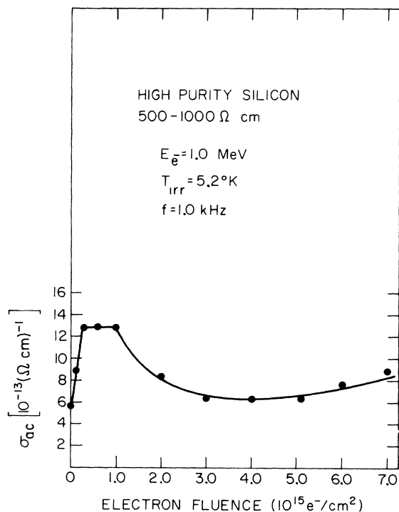
FIG. 20. Changes in \sigma_{ac} produced by irradiation of high-purity silicon at 5.2°K with 1.0-MeV electrons.
