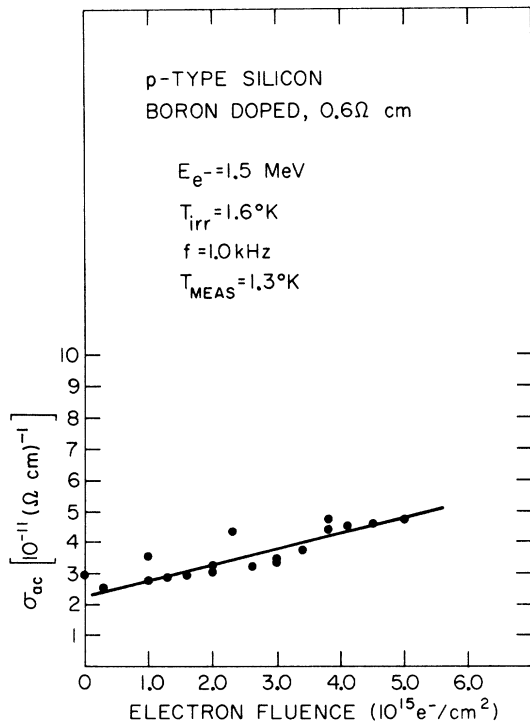
FIG. 9. Changes in \sigma_{ac} produced with irradiation at 1.6°K of 0.6- \Omega -cm boron-doped p -type silicon.
