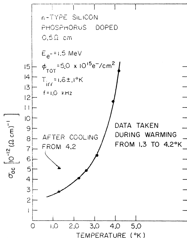
FIG. 16. Magnitude of \sigma_{ac} as a function of temperature measured at various temperatures during warming from 1.3 to 4.2 ^\circ K and back to 1.3 ^\circ K after end of irradiation.
